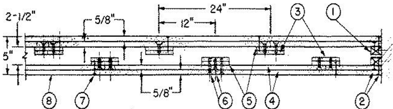
Horizontal Section
